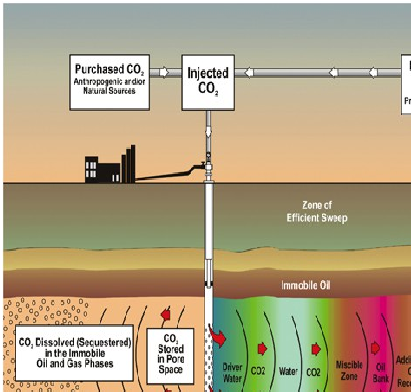
Fig.6 Enhanced Oil Recovery (EOR) (see endnote 12)
