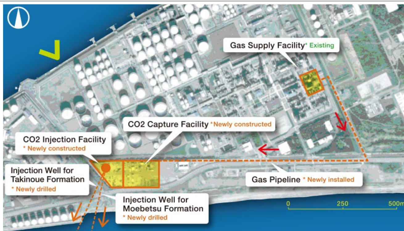
Fig. 5. CCS Demonstration Project at Tomakomai area in Hokkaido
